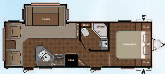
WEIGHT: 6070 LENGTH: 29' 7" 258RLWE
